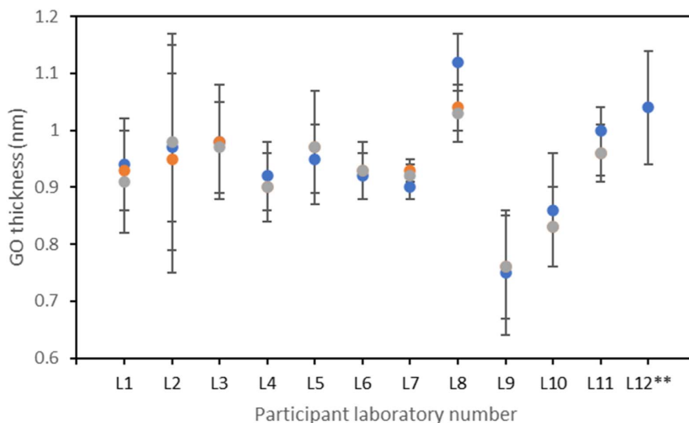
Figure 2. Participants' results for GO thickness using different data analysis methods: ● three height profiles* ● All height profiles ● Whole area. Note: *data obtained from participants; **raw data could not be analyzed with available algorithm software.
