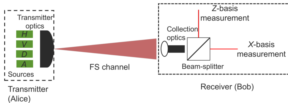
Figure 3. A common terrestrial based free space QKD system, an illustration [16].
