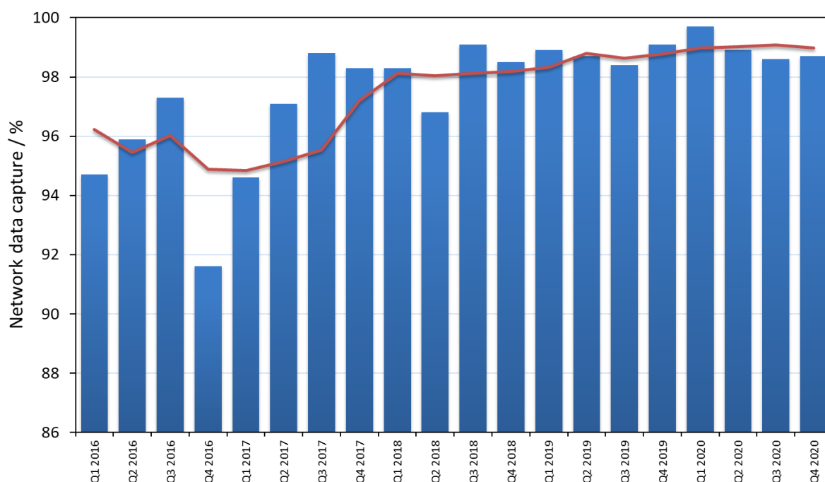
Figure 2 Network data capture from the last five years (2016-2020 inclusive) for particulate measurements. Quarterly data capture is indicated by the blue bars, whilst the rolling annual average data capture is given by the red line.
