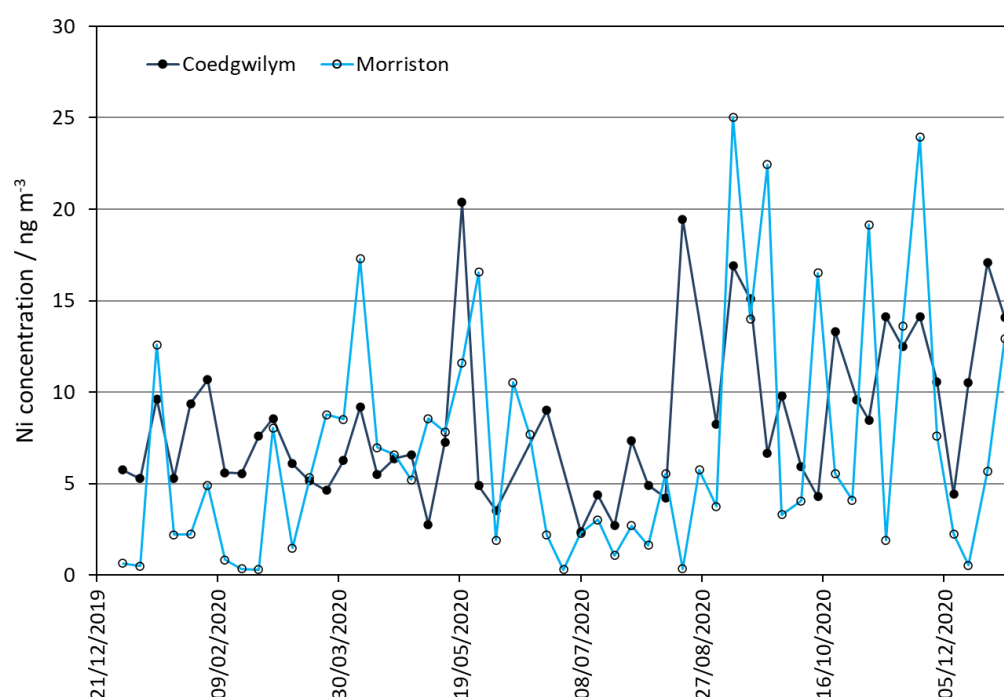
Figure 5 Measured Ni concentrations at Site 100: Swansea Coedgwilym and Site 101: Swansea Morriston, in 2020 (both sampled weekly).
