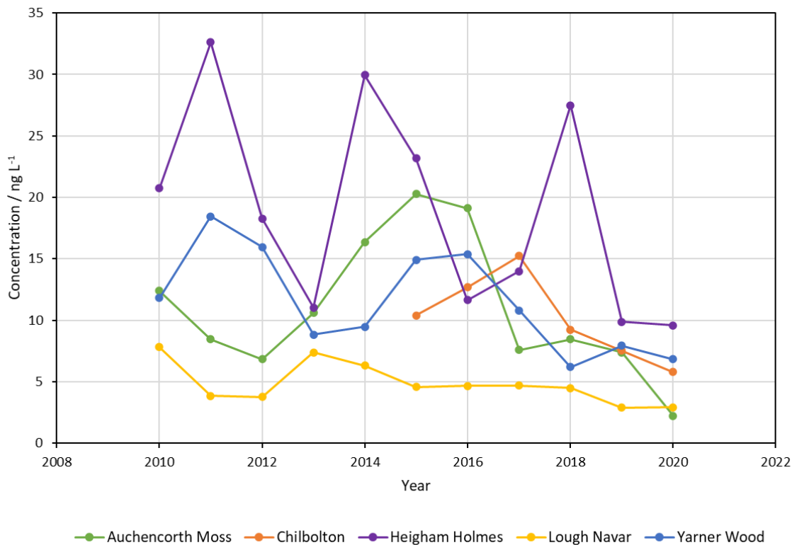
Figure 18 The mean annual concentrations of Cd measured in deposition since 2010 at individual sites.
