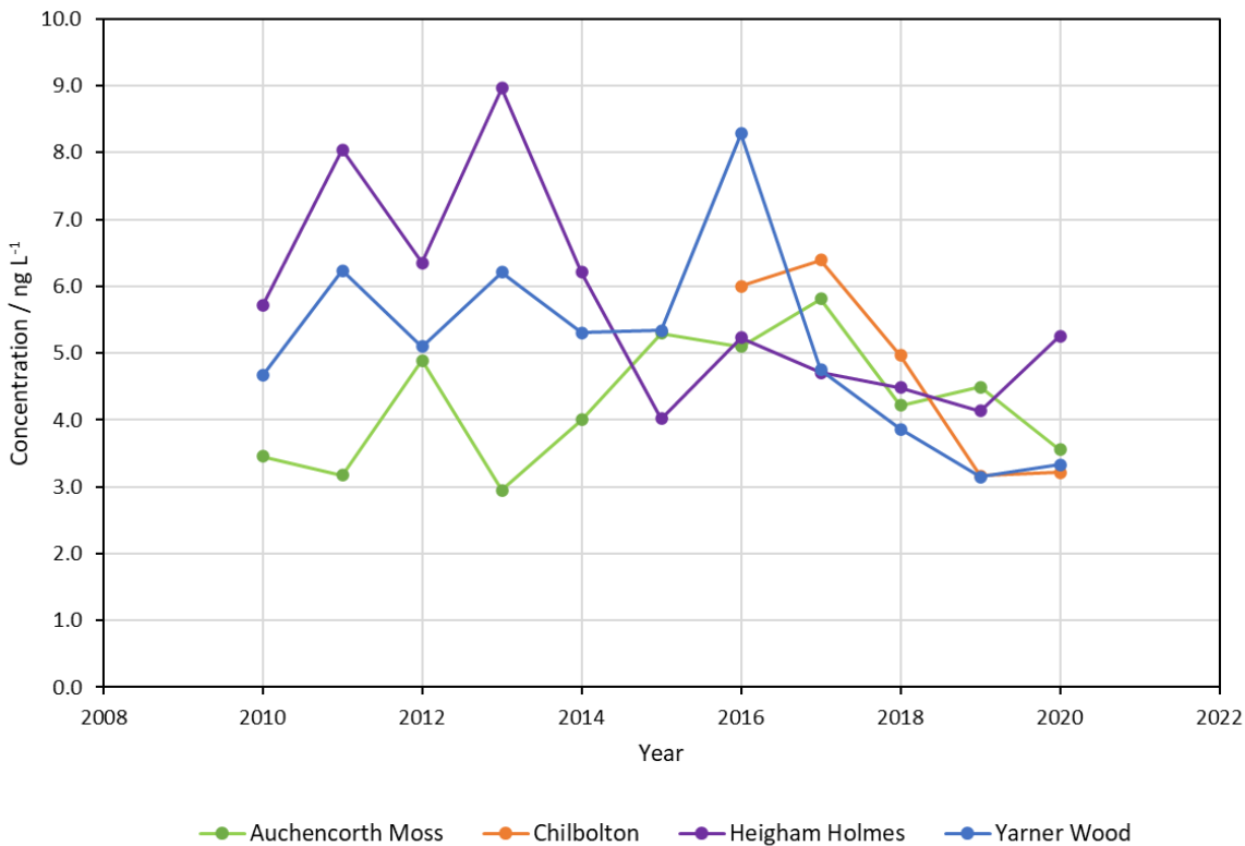
Figure 19 The mean annual concentrations of Hg measured in deposition since 2010 at individual sites. Hg is not measured at Lough Navar.
