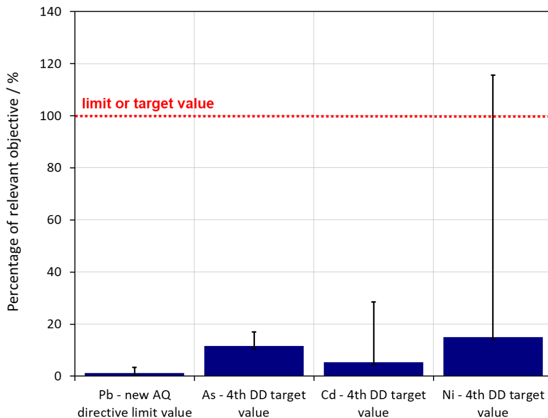
Figure 3 A summary of the annual mean measured concentrations of the heavy metals relevant to the Ambient Air Quality Directive and Fourth Daughter Directive on the UK Heavy Metals Monitoring Network in 2020 as a percentage of the relevant air quality objectives. The bars indicate the annual mean of all sites; the lines indicate the annual mean at the site with the highest concentrations.
