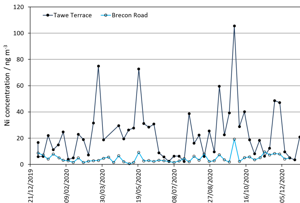
Figure 6 Measured Ni concentrations at Site 113: Pontardawe Tawe Terrace and Site 115: Pontardawe Brecon Road, in 2020 (both sampled weekly).
