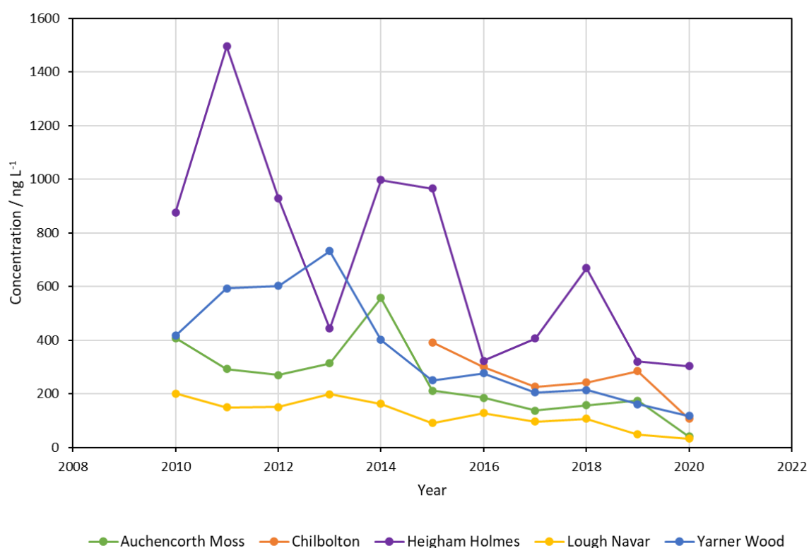
Figure 15 The mean annual concentrations of Pb measured in deposition since 2010 at individual sites.
