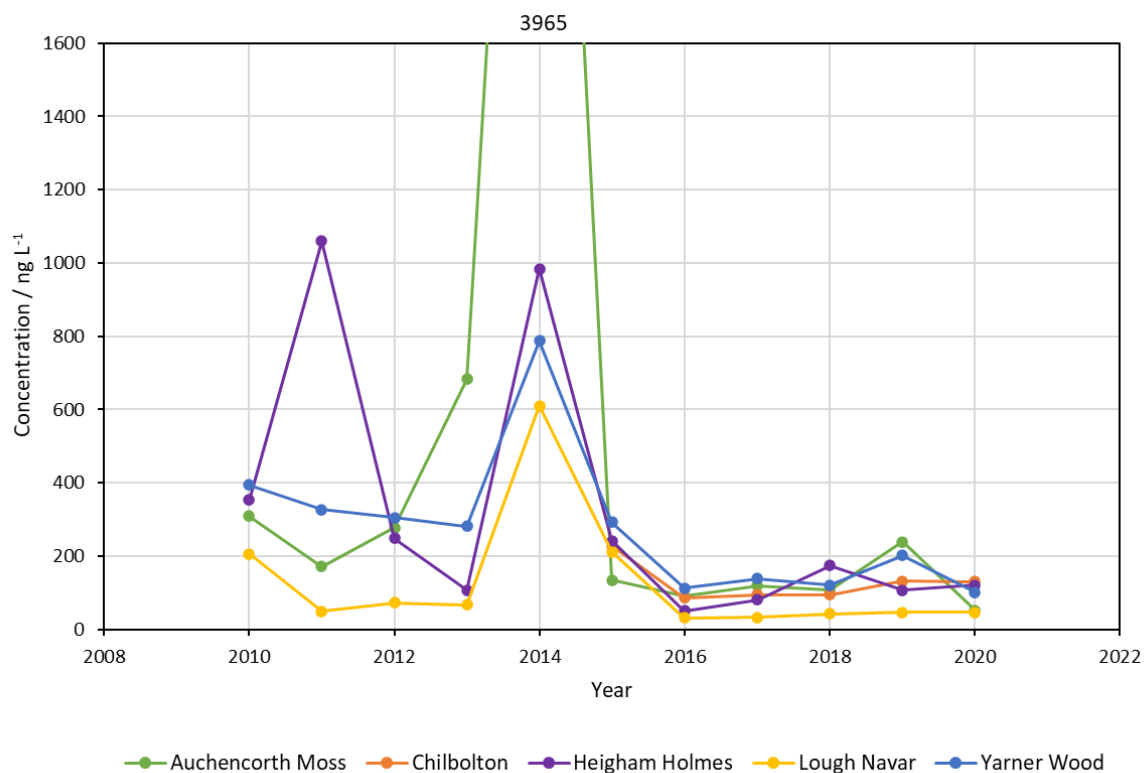
Figure 16 The mean annual concentrations of Ni measured in deposition since 2010 at individual sites.
