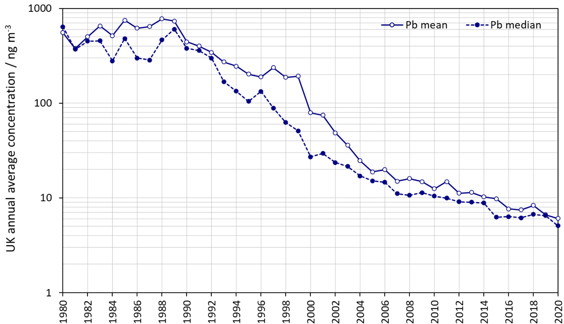
Figure 9 The mean and median of site annual average concentrations of Pb measured on the UK Heavy Metals Monitoring Network over the last 40 years. The EC limit value for lead is 500 \text{ ng m}^{-3} and the UK Air Quality Objective for lead is 250 \text{ ng m}^{-3} . Note the logarithmic scale on the y-axis.
