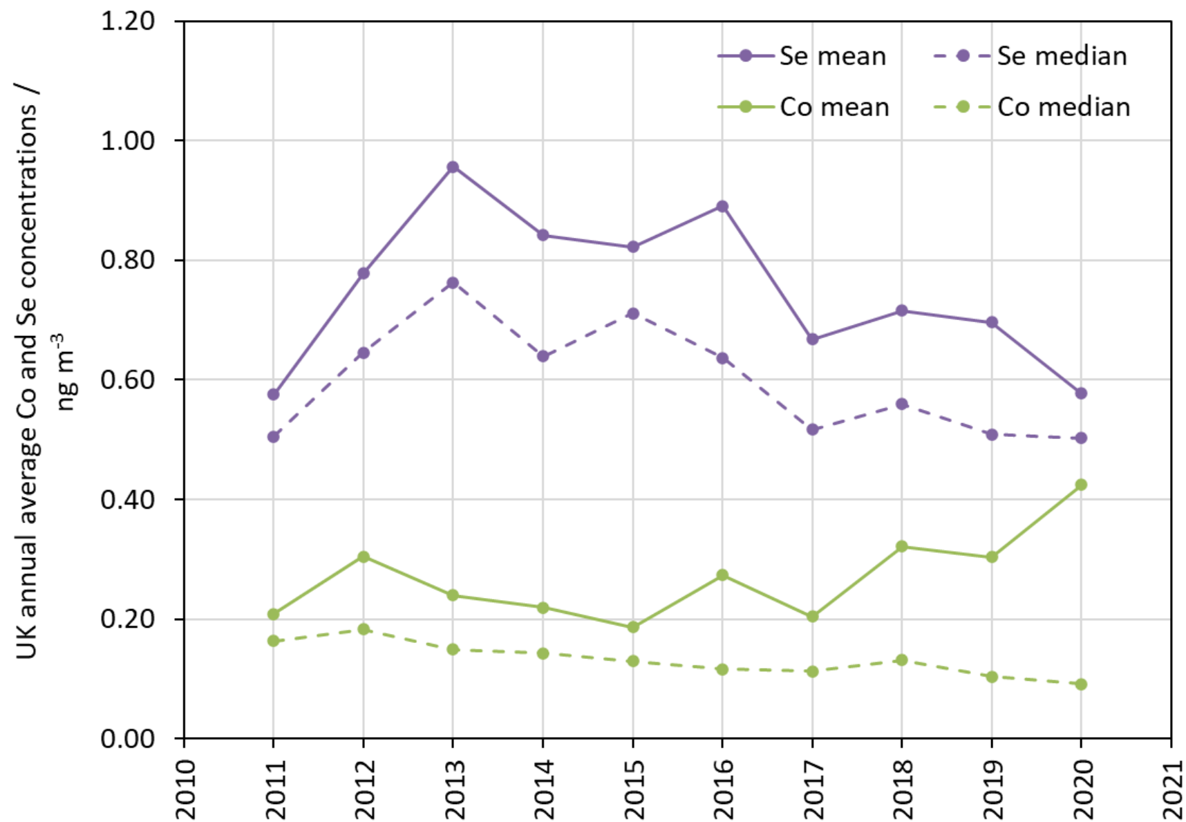
Figure 13 The mean and median of site annual average concentrations of Co and Se measured on the UK Heavy Metals Monitoring Network since monitoring commenced for these metals in 2011.
