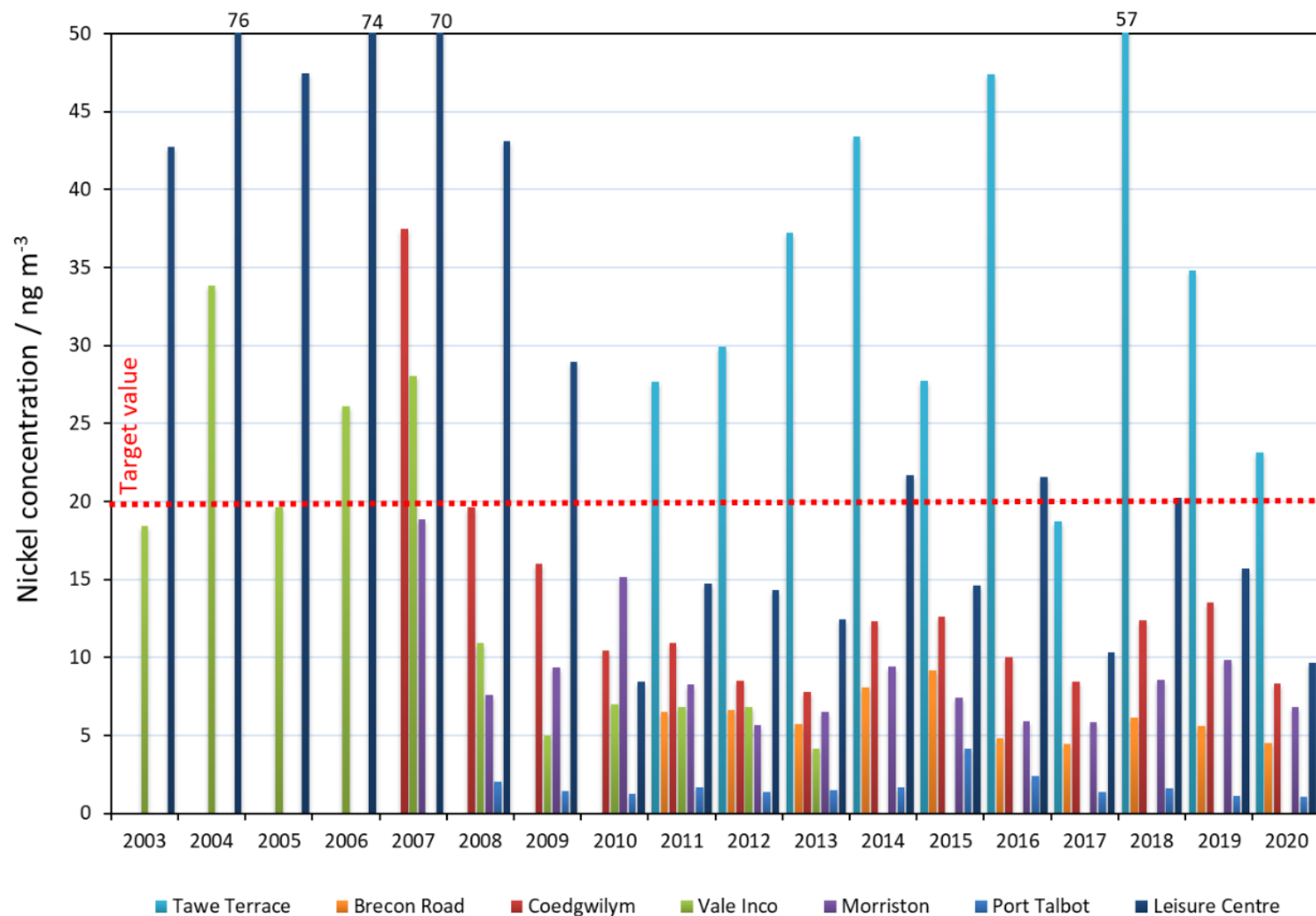
Figure 14 The annual average nickel concentrations measured at monitoring sites in the Swansea area 2003-20. The red dotted line indicates the Fourth DD target value for nickel.
