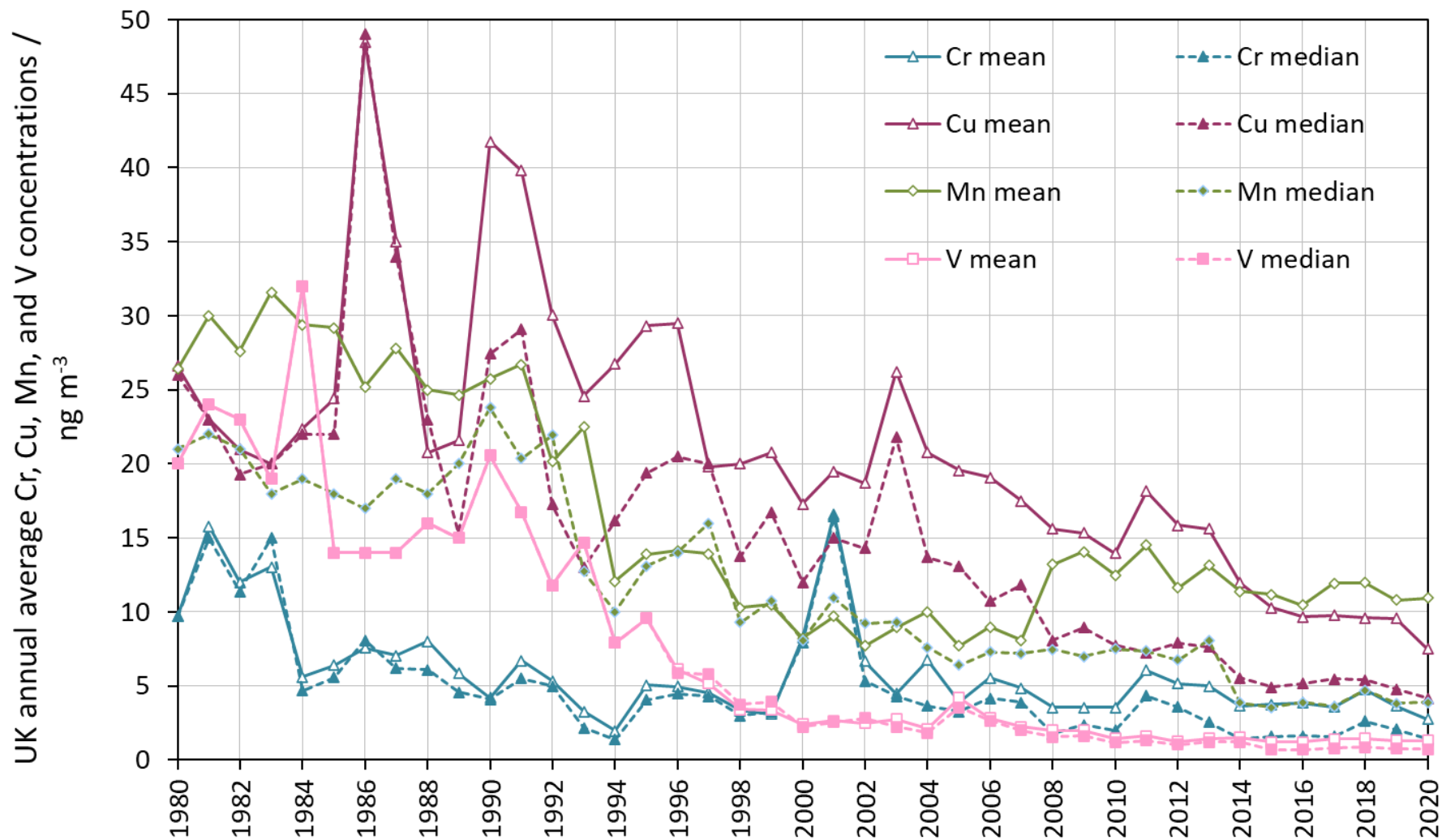
Figure 12 The mean and median of site annual average concentrations of Cr, Cu, Mn, and V measured on the UK Heavy Metals Monitoring Network over the last 40 years.
