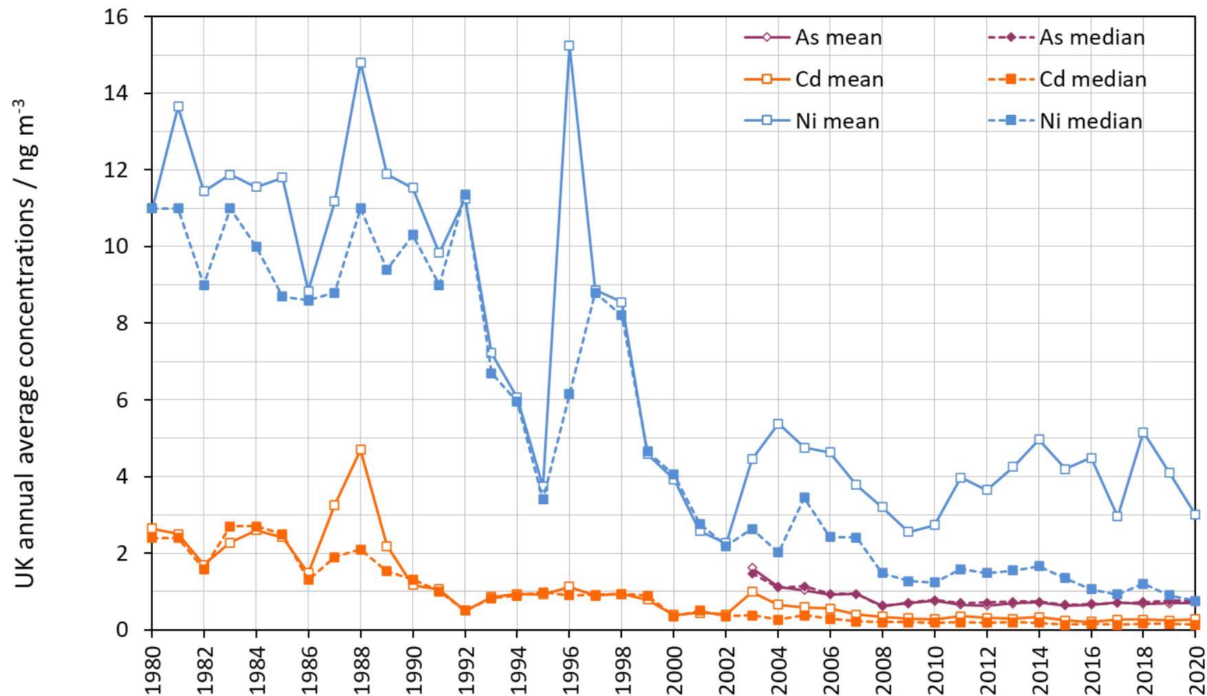
Figure 10 The mean and median of site annual average concentrations of Ni, As and Cd measured on the UK Heavy Metals Monitoring Network over the last 40 years. The EC target values for Ni, As and Cd are 20 \text{ ng m}^{-3} , 6 \text{ ng m}^{-3} and 5 \text{ ng m}^{-3} respectively.
