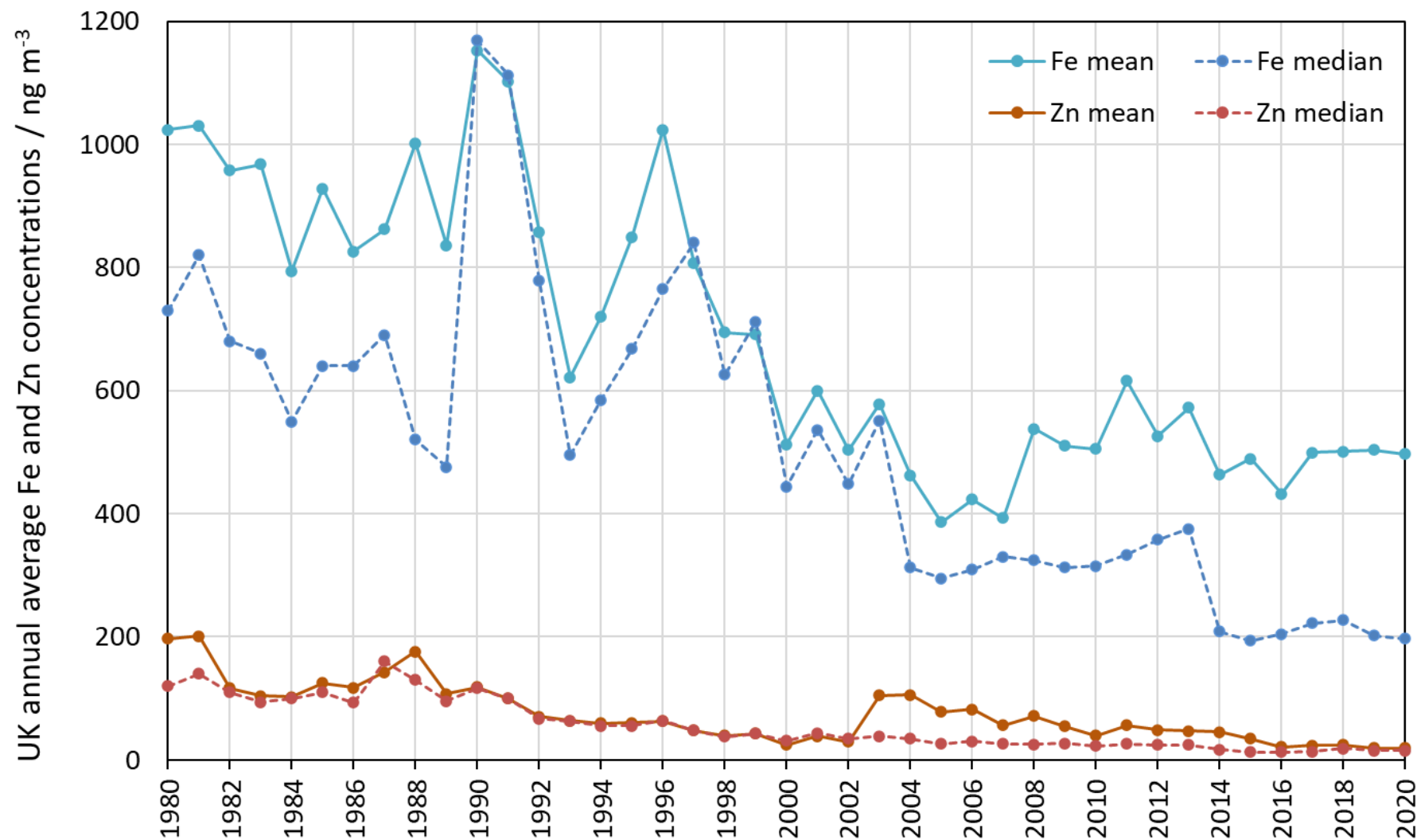
Figure 11 The mean and median of site annual average concentrations of Fe and Zn measured on the UK Heavy Metals Monitoring Network over the last 40 years.
