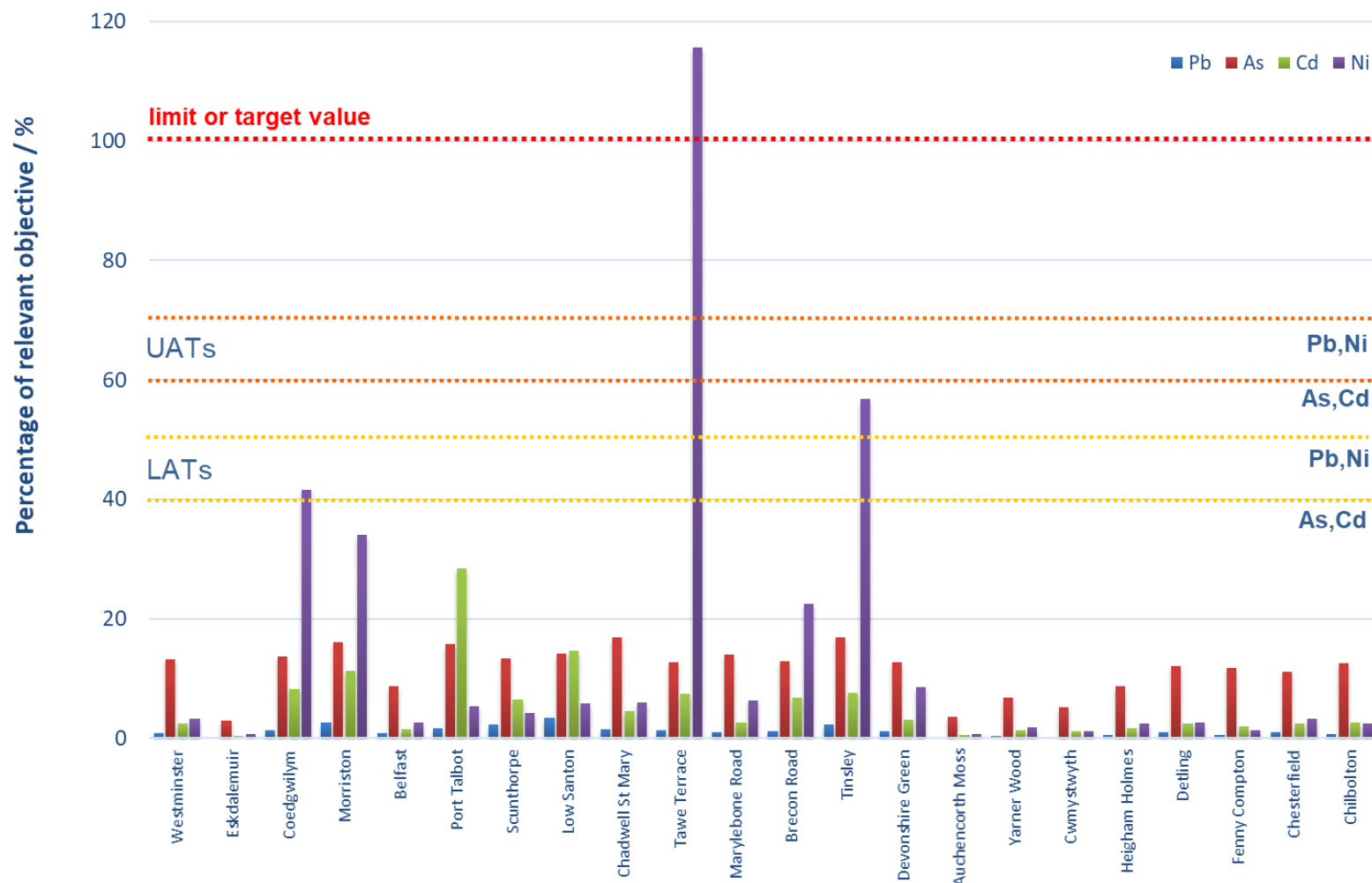
Figure 4 A summary of the annual mean measured concentrations of the heavy metals relevant to the New Air Quality Directive and Fourth DD at all sites on the UK Heavy Metals Monitoring Network in 2020 as a percentage of the relevant target values shown in red, upper assessment thresholds (UATs) in orange and lower assessment thresholds (LATs) in yellow.
