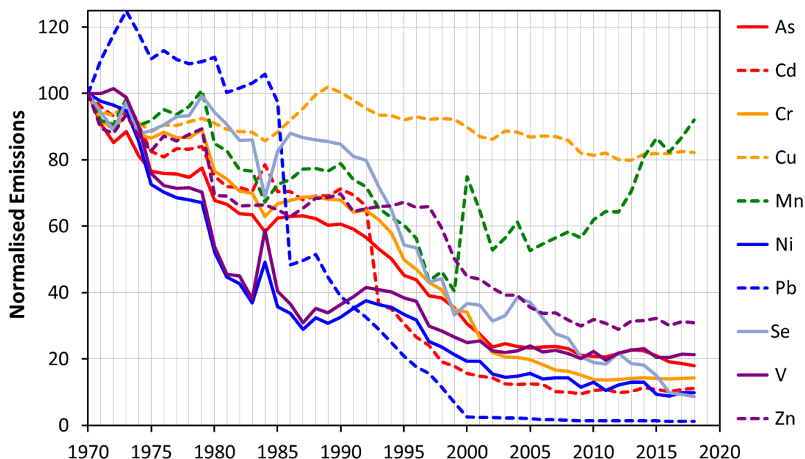
Figure 1 Estimated UK annual emissions of the metals from 1970 to 2018 6 (the latest year for which emissions data were available at time of publishing) normalised to their values in 1970. The absolute levels of emissions in 1970, in tonnes, were: As, 81; Cd, 36; Cr, 254; Cu, 327; Mn, 89; Ni, 989; Pb, 7492; Se, 92; V, 2749; and Zn, 1482. Emissions data are not available for Co or Fe, although these are measured by the Network.
