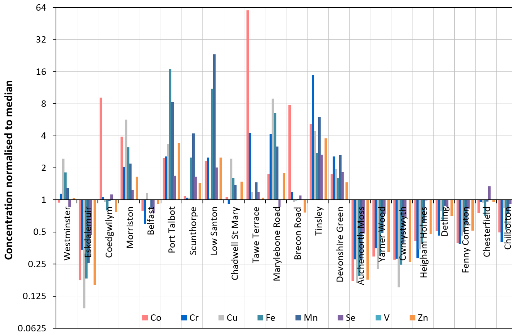
Figure 8 A summary of the annual mean measured concentrations of the non-directive metals at all sites on the UK Heavy Metals Monitoring Network in 2020, normalised to the UK annual median concentration for the relevant element. These values are plotted with respect to the median, so it is clear which sites are above and below the median level. Note the logarithmic scale on the y-axis.
