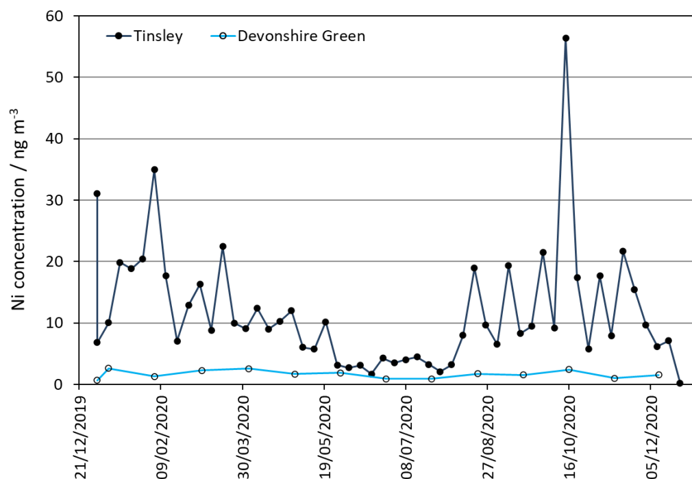
Figure 7 Measured Ni concentrations at Site 117: Sheffield Tinsley and Site 119: Sheffield Devonshire Green in 2020. Sampling at Tinsley is weekly. Results from Sheffield Devonshire Green are averaged over four-week periods.
