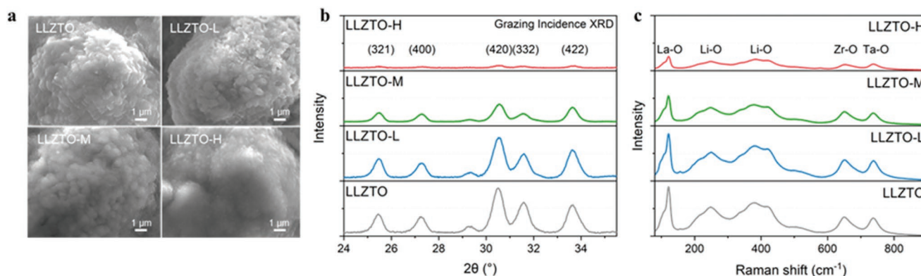
Figure 4. a) Surface morphologies, b) GI-XRD patterns, and c) Raman spectra of the LLZTO pellet and the pellets after the different doses of Xe ion implantation. All instrument parameters are the same for each sample, all pellet bodies come from the same preparation method, and all the patterns are drawn in the same scale.
