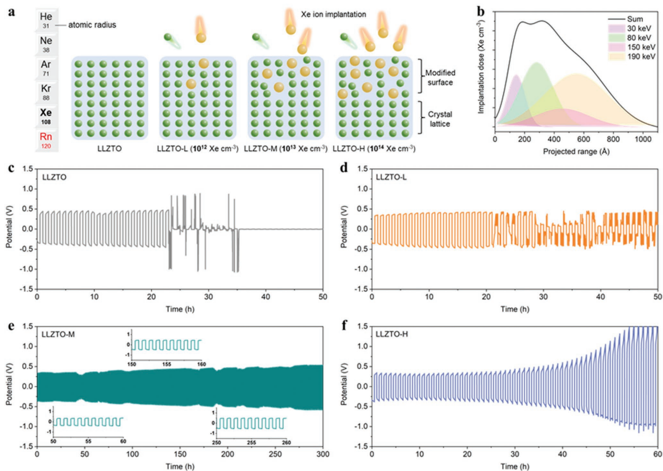
Figure 3. a) Schematic illustration of the Xe ion implantation and atomic radius table for noble gases. b) Projected range distribution for each accelerating voltage and overall weighted distribution for the Xe ion implantation. Galvanostatic cycling performance of the lithium plating/stripping in the symmetric lithium cells assembled with c) LLZTO, d) LLZTO-L, e) LLZTO-M, and f) LLZTO-H at room temperature (current density: 0.1 \text{ mA cm}^{-2} ).
