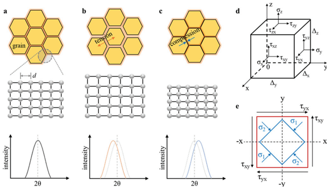
Figure 1. a–c) The top row gives representations of a) unstressed reference, b) tensile stress, and c) compressive stress. The middle row and the bottom row indicate the signatures of each stress states in lattice and diffraction patterns, respectively. d) Schematic diagram of stresses acting on an elemental unit. e) Sign convention for shear stresses and illustration of principal stress in a global coordinate system for a pure shear case.
