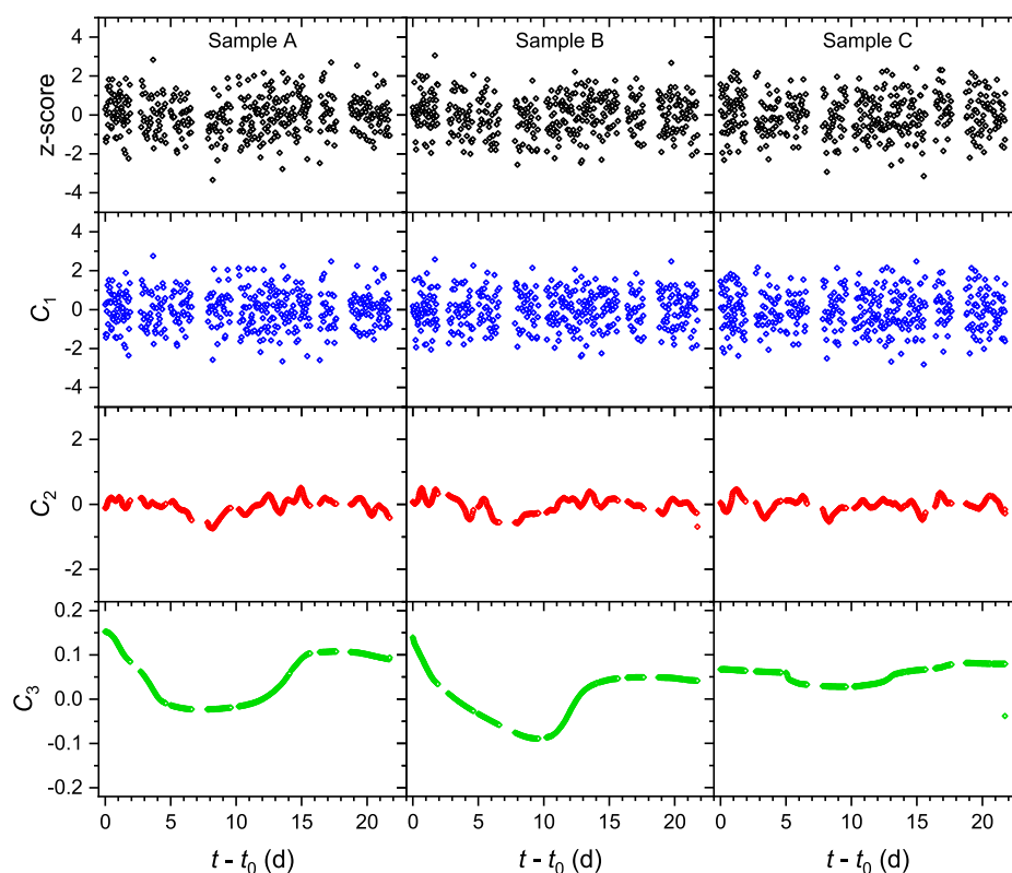
Fig. 10. Empirical mode decomposition of the residuals to the least-squares fit to samples A, B, and C data sets measured by the HIDEK 300SL liquid scintillation counter. The random statistical component ( C_1 ), a medium-frequency ( C_2 ), and a slow-frequency remainder ( C_3 ) component are shown.
