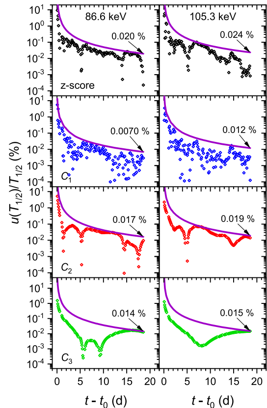
Fig. 7. The relative uncertainty of the half-life for the decomposition modes C_1 , C_2 and C_3 as a function of time for the 86.6 keV (left) and 105.3 keV (right) residuals. The purple line represents their envelope function, with their ultimate uncertainty values indicated. (For interpretation of the references to colour in this figure legend, the reader is referred to the Web version of this article.)
