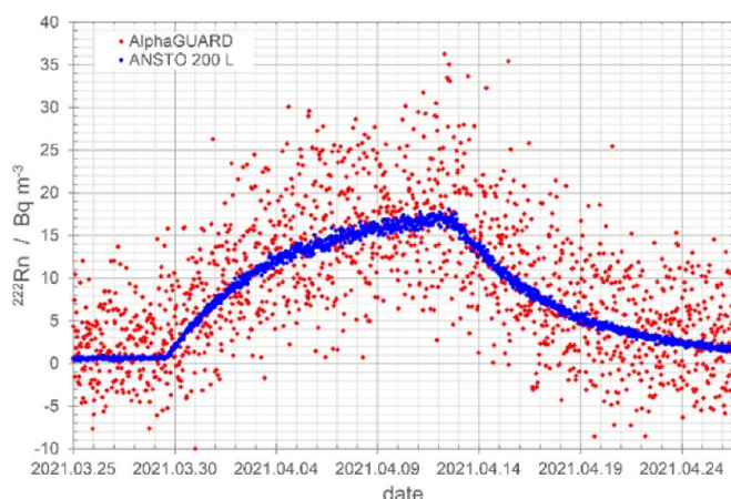
Figure 2. A low-level calibration situation in a non-constant atmosphere: the adjusted response of two types of detectors (AlphaGuard in red, ANSTO 200 l in blue) in a build-up and decay situation in a closed large-volume climate chamber at PTB.
