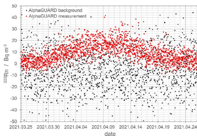
Figure 3. A low-level calibration situation in a non-constant atmosphere: One AlphaGuard in red from figure 2 in a build-up and decay situation in a closed large volume climate chamber at PTB. The activity concentration outside the climate chamber is given by a second AlphaGuard in black.
