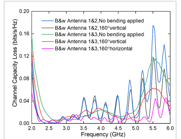
Figure 11. Channel capacity loss between antennas with and without being bent calculated from measured scattering parameters.
