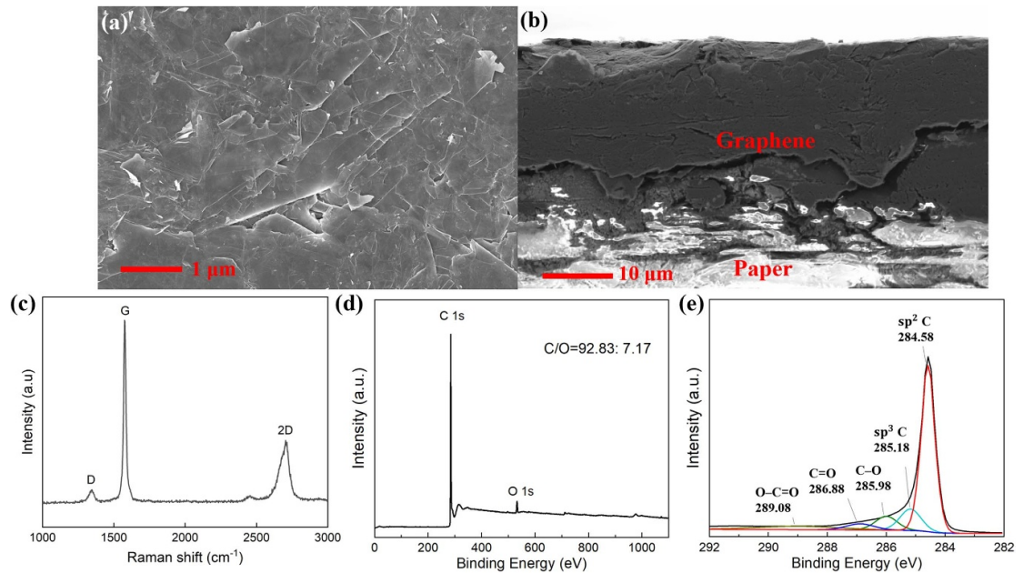
Figure 1. (a) 10k× magnified SEM top view of the screen-printed graphene surface with 1 \mu\text{m} scaled bar. (b) 500× magnified SEM cross-sectional view of the antenna with 10 \mu\text{m} scaled bar, the average thickness of the graphene laminate is 19.4 \mu\text{m} . (c) Raman spectra of printed graphene, (d) wide-scan XPS spectra and (e) deconvolution of C 1s XPS spectra of the printed graphene.
