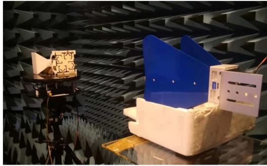
Figure 6. Antenna measurement set up with a horn antenna in anechoic chamber, the distance between the horn antenna and the MIMO antenna under test is 0.8 m.
