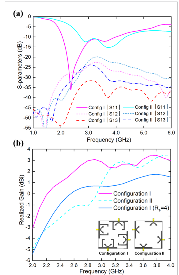
Figure 5. Comparison of simulated results for (a) S-parameters and (b) realized gain of two different configurations (with and without ground extension stubs).
