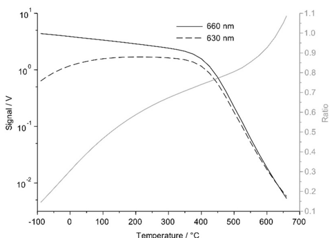
Figure 6. Signal levels from the two detectors (black lines and scale) and their ratio (grey line and scale).
