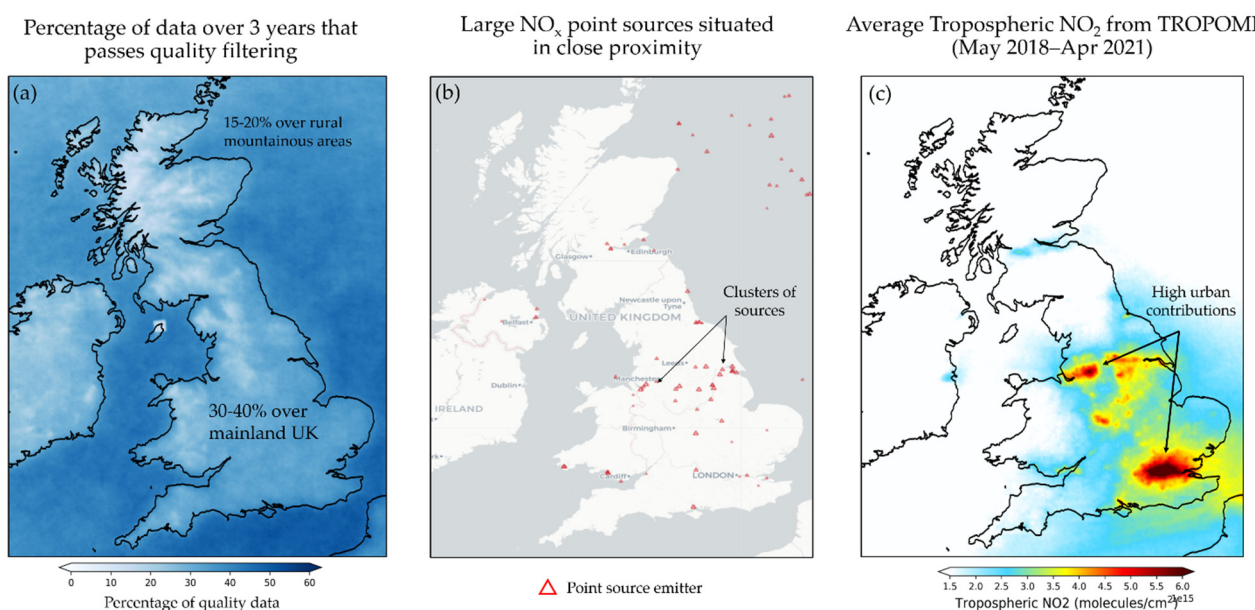
Figure 1. Three plots demonstrating the difficulties associated with retrievals over the UK. (a) The percentage of TROPOMI NO 2 observations that pass the quality filtering requirement of >0.75 and cloud radiance fraction <0.5, over a 3 year period from May 2018 to April 2021. (b) Location of large point source NO 2 emitters from the NAEI 2019 point source inventory. (c) The 3 year average of tropospheric NO 2 from TROPOMI from May 2018 to April 2021.
