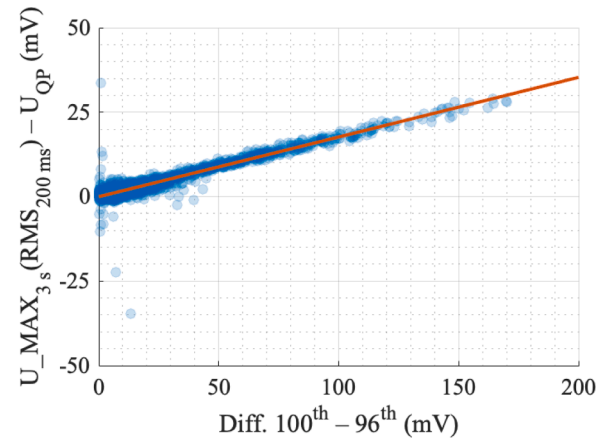
Fig. 3. Linear relationship between the outputs of the RM-A method and the CISPR 16-1-1.
