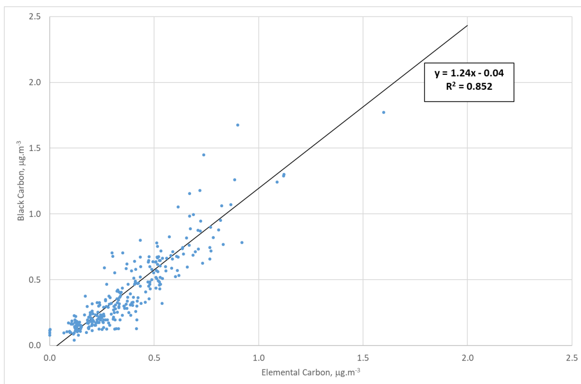
Figure 36 2018 EC and BC Measurements at Chilbolton
