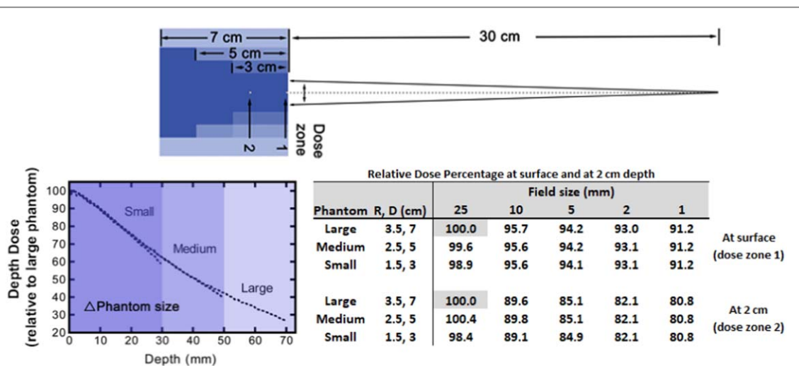
Figure 12. Depicts the influence of scatter on object and beam size in differing cylindrical geometries having an equal width/depth of 3, 5, or 7 cm and an SSD of 30 cm irradiated with the EGSnrc 250 kVp spectrum. The resulting percent depth dose (relative to the large phantom) shows that the percent depth dose is hardly affected when the phantom size changes. The percent depth dose also illustrates that at the exit of the beam, depth dose values deviate from a (larger) object reference. The embedded table provides relative dose percentages for phantoms and field sizes relative to large phantom with 25 mm field at surface and at 2 cm depth (both shaded in grey) for the two dose zones. The table illustrates that depth doses at orthovoltage energies are more sensitive to changes in field size than changes in object size. These values are only indicative and should be evaluated for other geometries and energies.
