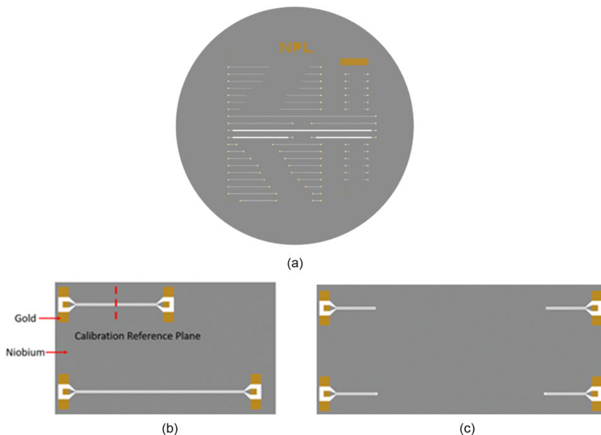
Figure 9. CAD drawing (a) layout of cryogenic on-wafer calibration standards; (b) thru, including reference plane indicator (top) and line (bottom); and (c) reflect standards: open (top) and short (bottom).
